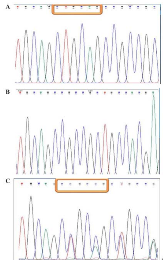
Figure 4. Direct sequencing of exon 1. A: homozygote for the 6bp insertion, B: homozygote without the insertion, C: heterozygote for the 6bp insertion
